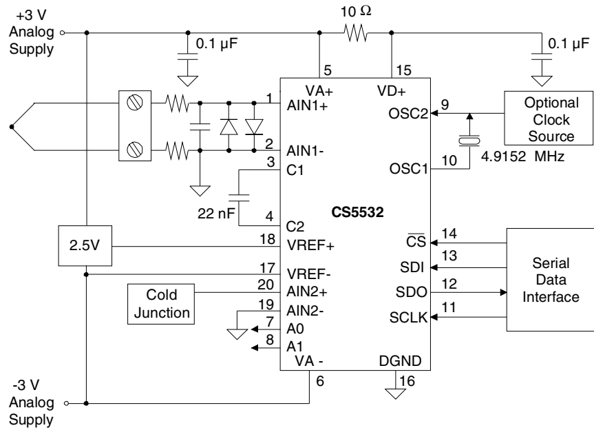
Figure 24. CS5532 Configured for Thermocouple Measurement
