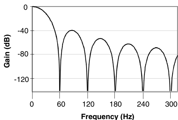
Figure 16. Digital Filter Response (Word Rate = 60 Sps)
