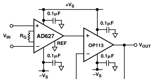
Figure 7. Output Buffering
