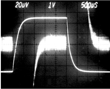
TPC 18. Large Signal Pulse Response and Settling Time, G = -1000 , R_L = 20\text{ k}\Omega , C_L = 100\text{ pF} ( 10\text{ }\mu\text{V} = 0.01\% )
