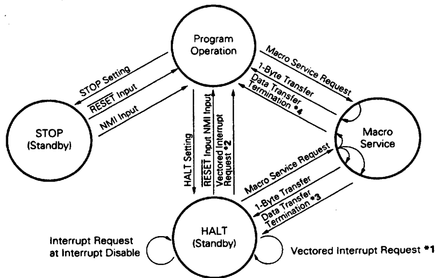
Fig. 4-4 Standby Status Flow
