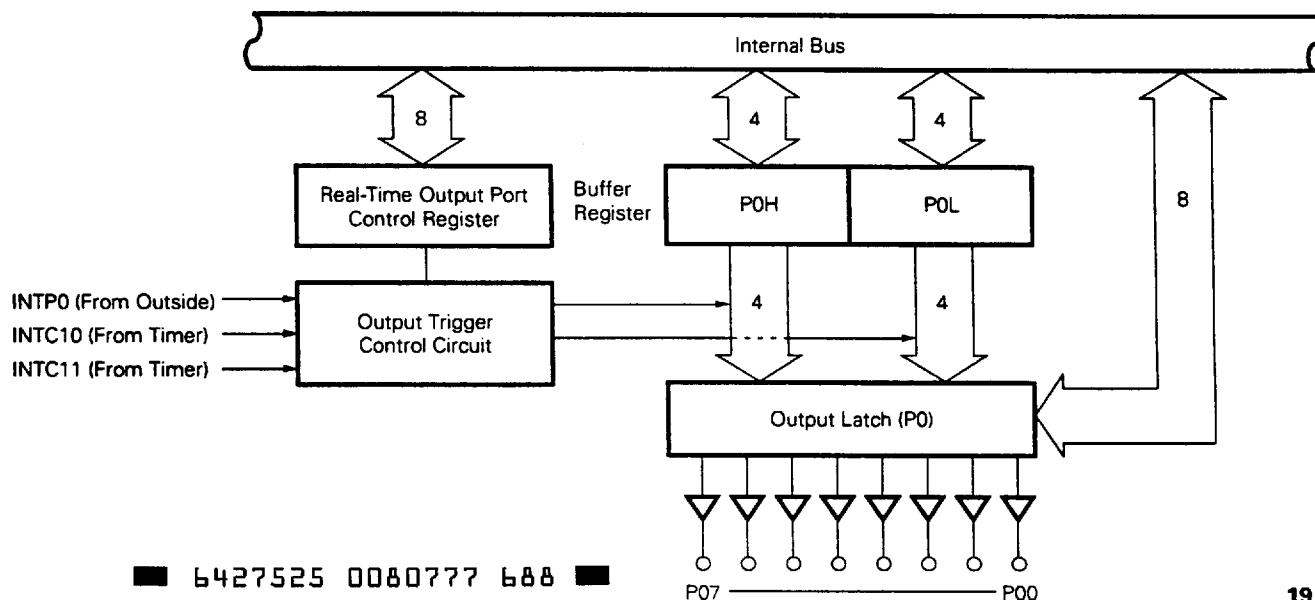
Fig. 3-4 Real-Time Output Port Block Diagram
