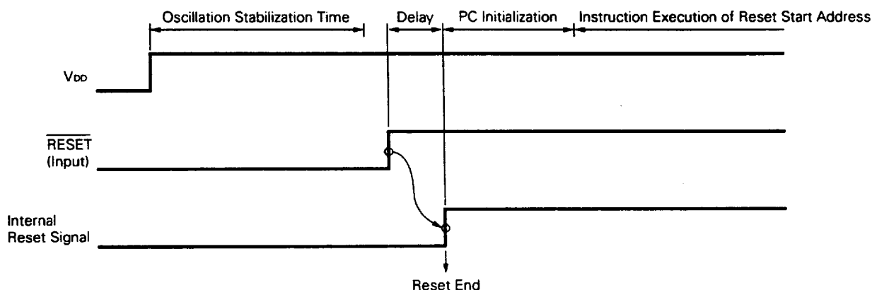
Fig. 4-6 Reset Operation at Power-On
