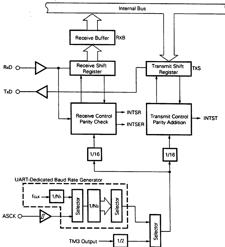
Fig. 3-8 Asynchronous Serial Interface Block Diagram
