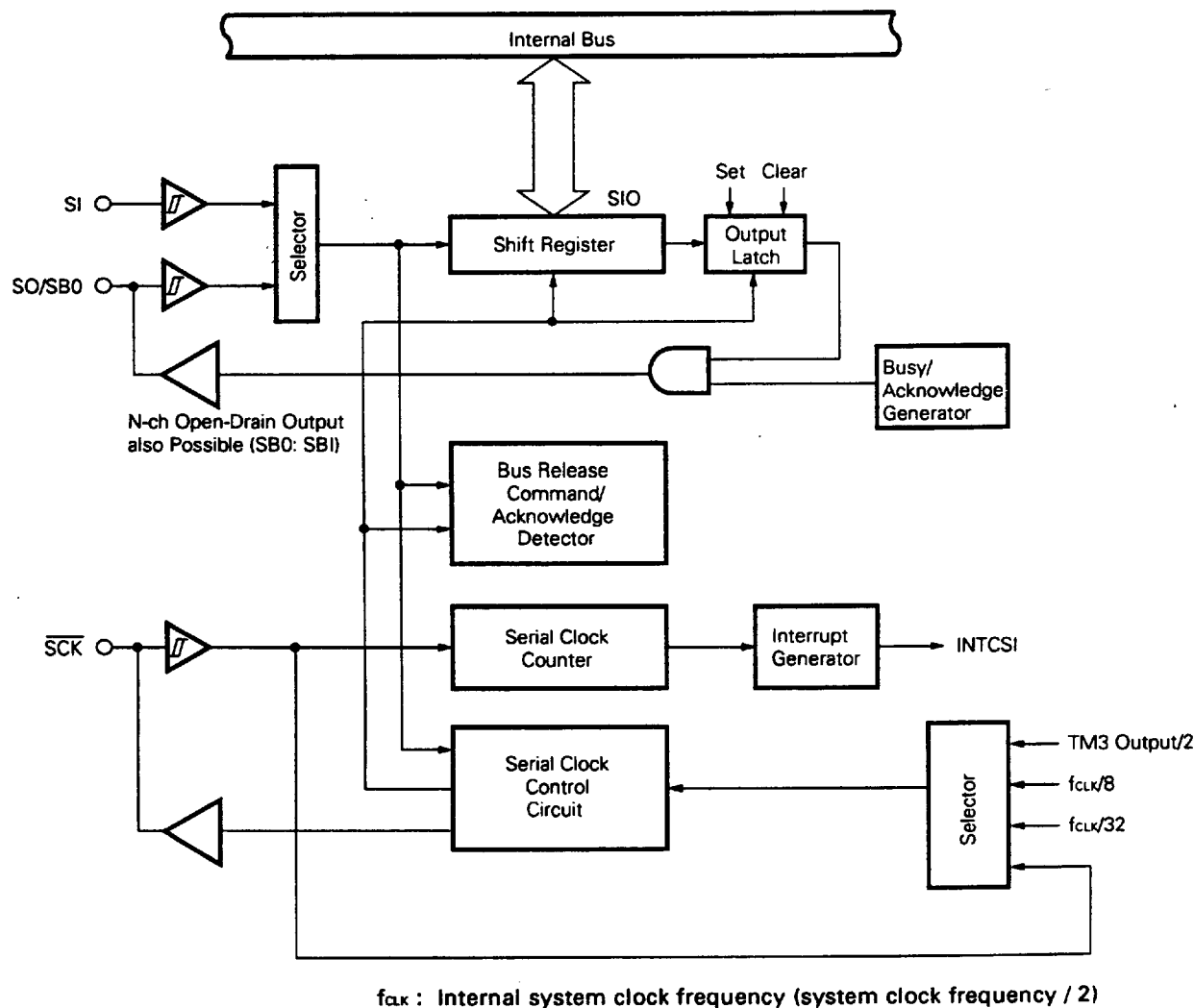
Fig. 3-9 Clocked Serial Interface Block Diagram
