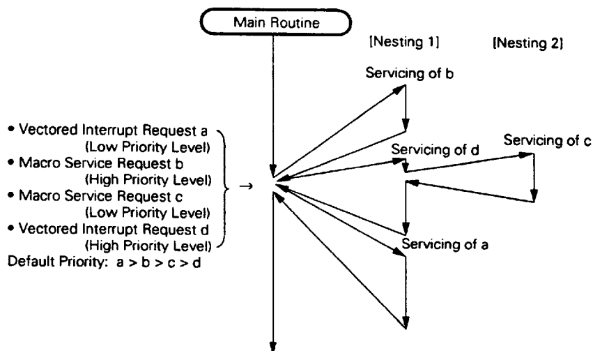
Fig. 4-2 Servicing Example for Simultaneously Generated Interrupt Request
