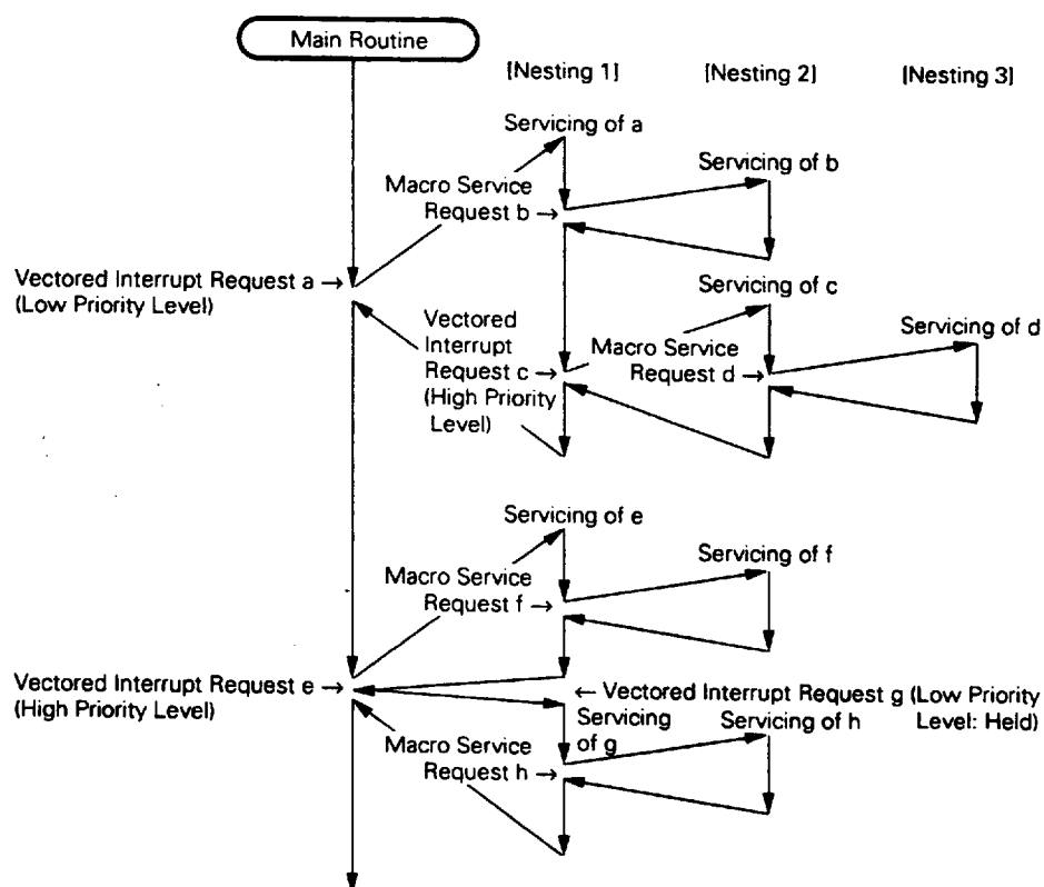
Fig. 4-1 Servicing Example for Another Interrupt Request Generation while an Interrupt Servicing
