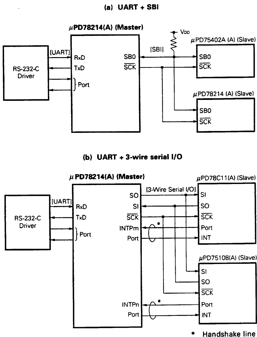
Fig. 3-7 Example of Serial Interface
