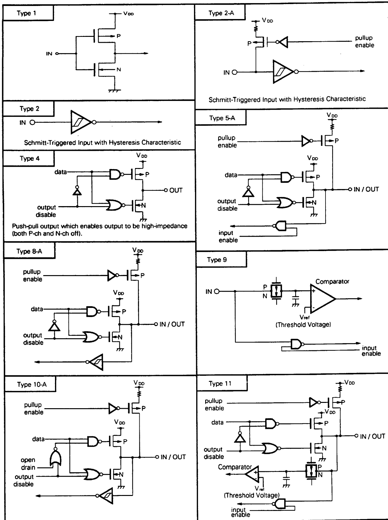
Fig. 2-1 Pin Input/Output Circuits
