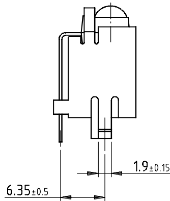
View "A"
