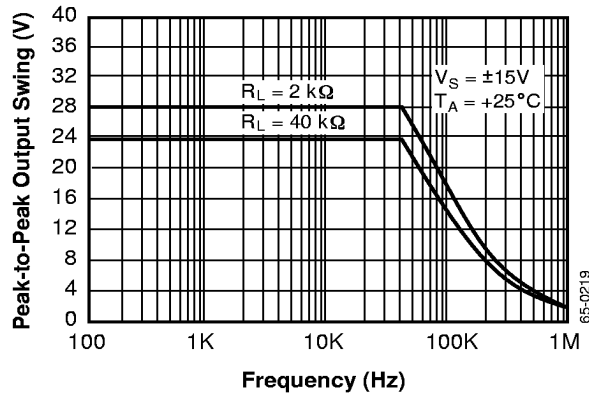
Output Voltage vs. Frequency
