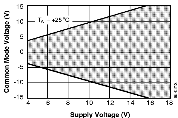
Common Mode Range vs. Supply Voltage
