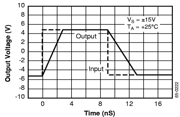
Voltage Follower Large Signal Pulse Response
