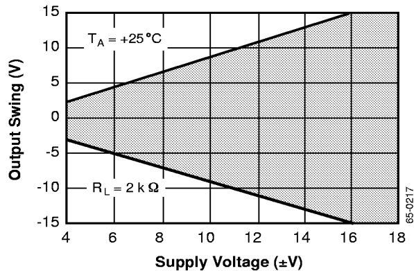
Typical Output Voltage vs. Supply Voltage
