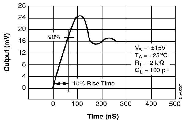
Transient Response
