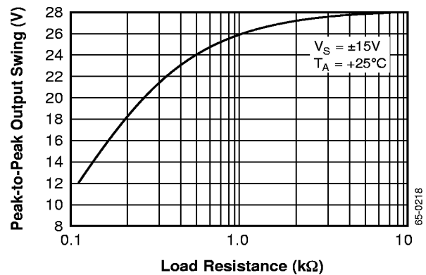
Output Voltage Swing vs. Load Resistance
