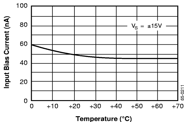
Input Bias Current vs. Ambient Temperature
