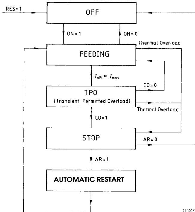
Figure 6 Line Driver State Diagram
