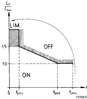
Figure 4 Diagram of the Transient Permitted Overload (TPO) State
