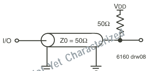
Figure 11. AC Termination
