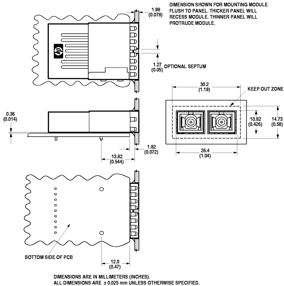
Figure 9. Suggested Module Positioning and Panel Cut-out for HFBR/HFCT-53D3FM.
