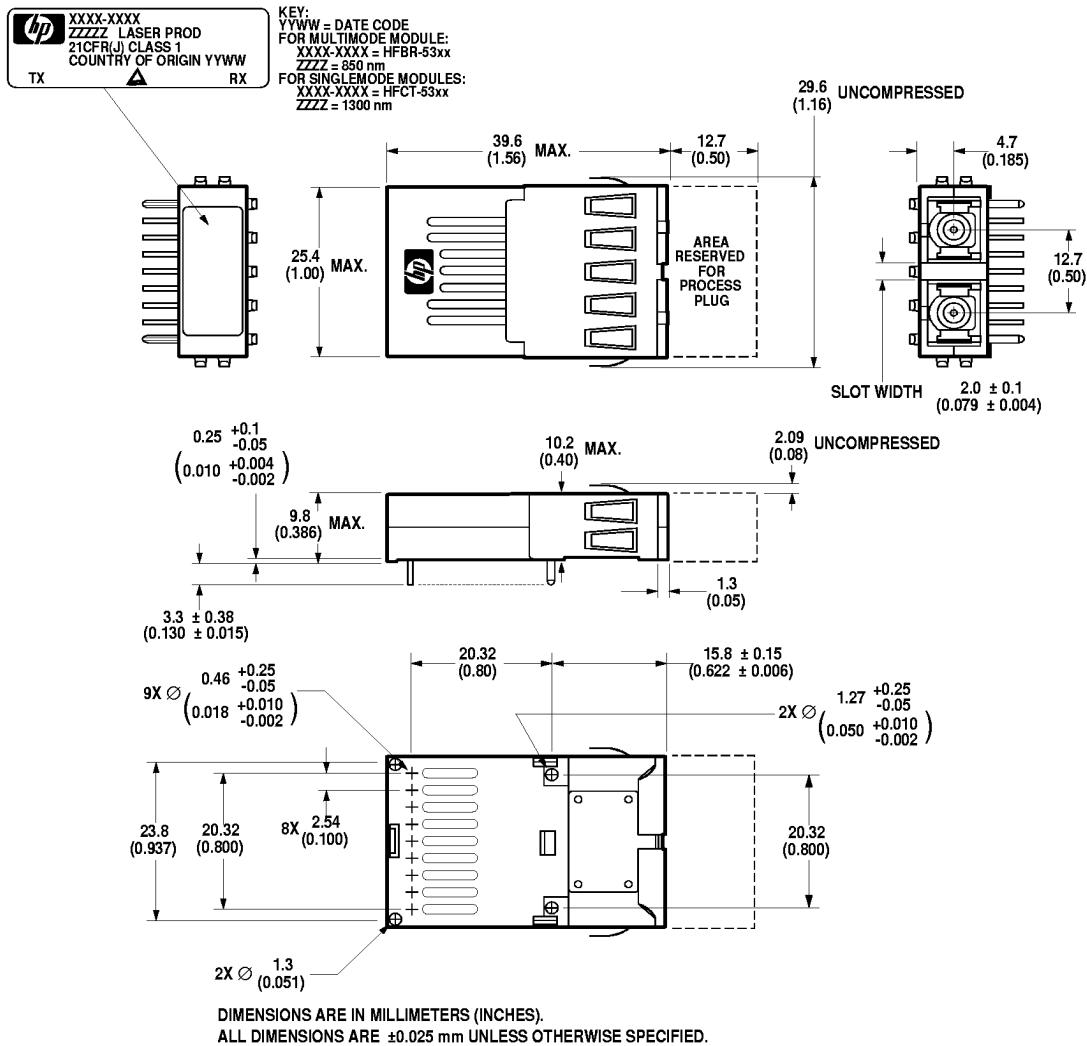
Figure 6. Package Outline for HFBR/HFCT-53D3EM.
