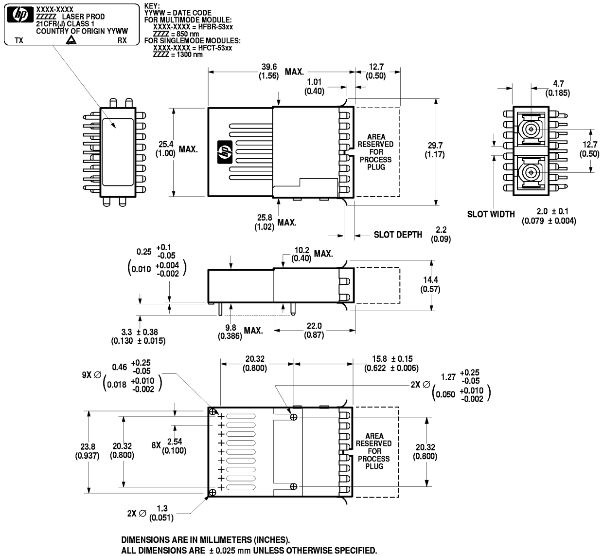
Figure 8. Package Outline for HFBR/HFCT-53D3FM.
