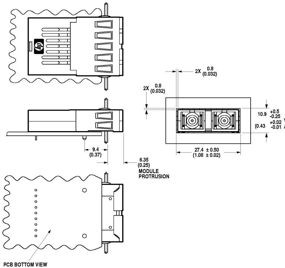
Figure 7. Suggested Module Positioning and Panel Cut-out for HFBR/HFCT-53D3EM.
