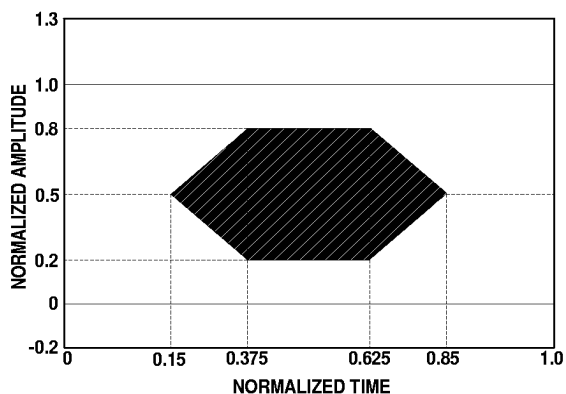
Figure 1. Transmitter Optical Eye Diagram Mask
