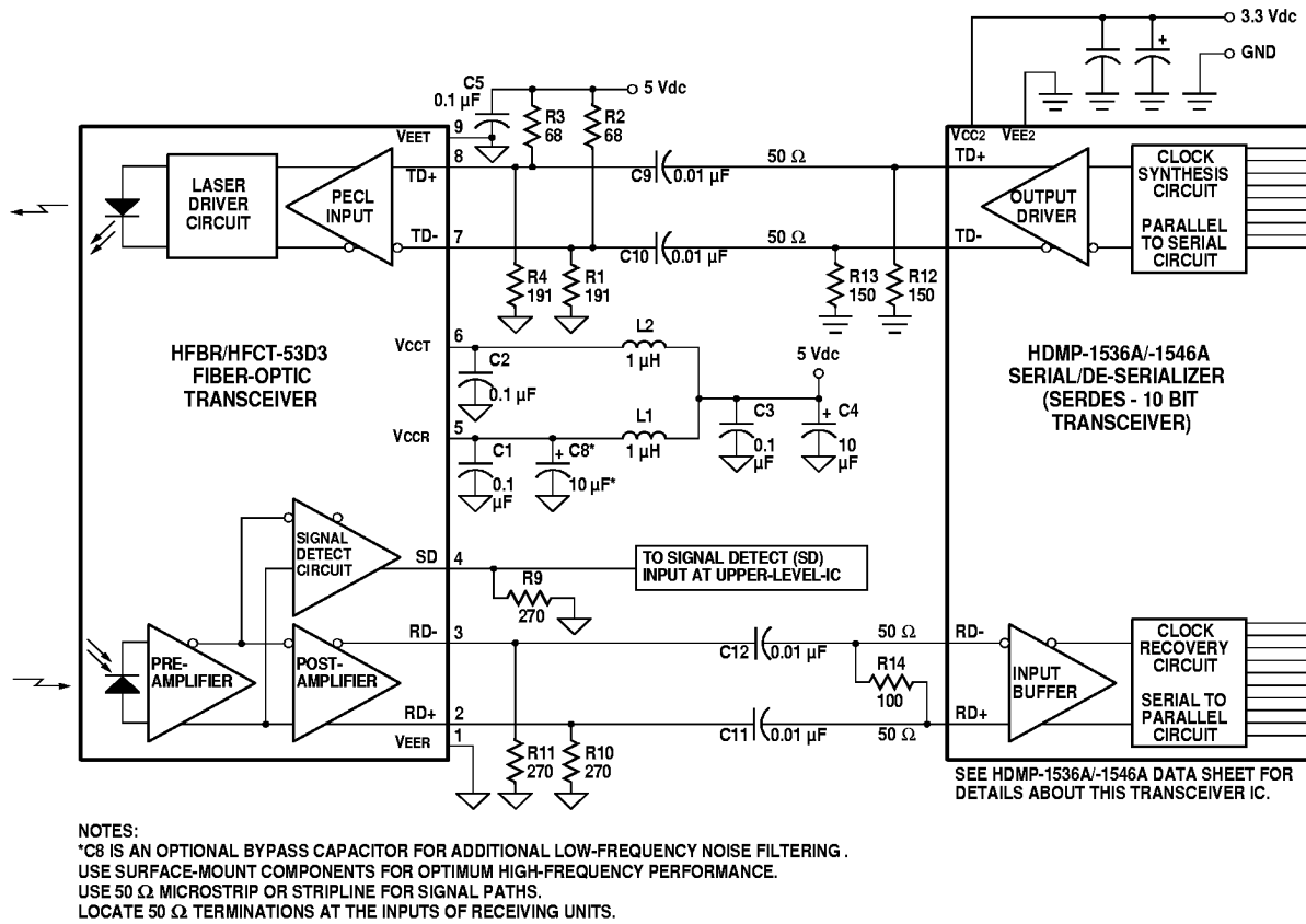
Figure 3. Recommended Gigabit/sec Ethernet HFBR/HFCT-53D3 Fiber-Optic Transceiver and HDMP-1536A/1546A SERDES Integrated Circuit Transceiver Interface and Power Supply Filter Circuits.
