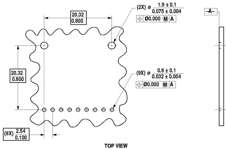
Figure 4. Recommended Board Layout Hole Pattern.
