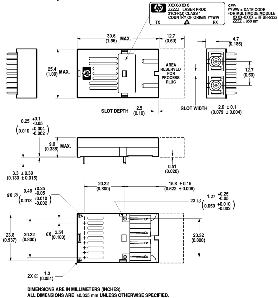
Figure 5. Package Outline Drawing for HFBR/HFCT-53D3.
