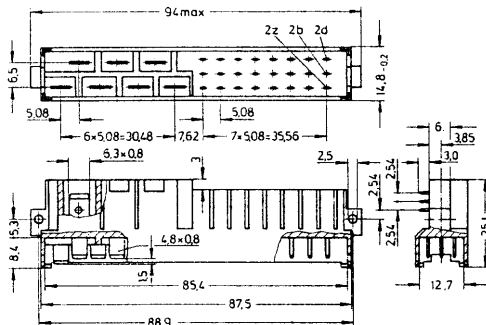
Faston terminal
