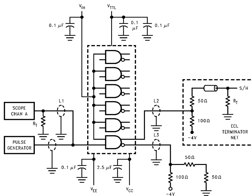
FIGURE 1. Propagation Delay and Transition Times
