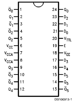
24-Pin DIP
