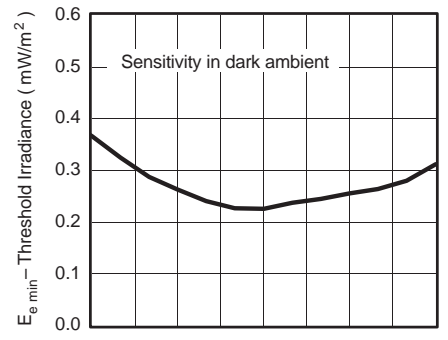
16918 T_{amb} - Ambient Temperature ( ^{\circ}C )
