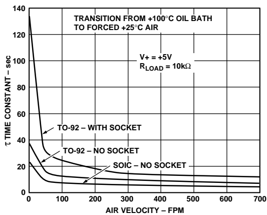
Figure 23. Thermal Time Constant in Forced Air
