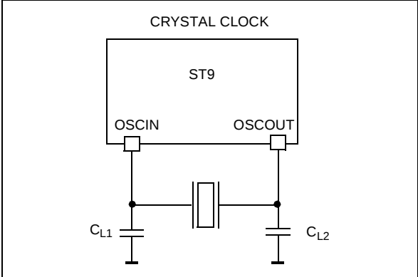
Figure 29. Crystal Oscillator
