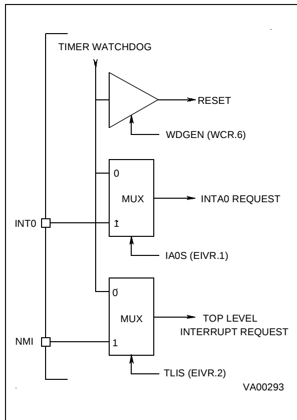
Figure 45. Interrupt Sources
