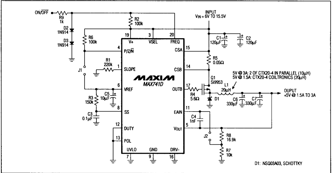
Figure 7. MAX741D EV Kit Schematic. +6V to +15.5V Input Step-Down Converter Supplies +5V at 1.5A or 3A.
