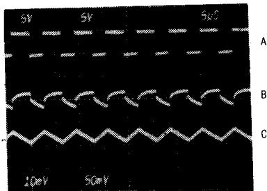
A = MOSFET DRAIN VOLTAGE (5V/div) B = OUTPUT VOLTAGE RIPPLE (AC: 50mV/div) C = INDUCTOR CURRENT (1A/div) CIRCUIT OF FIGURE 7
