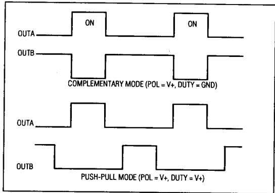
Figure 2. Push-Pull and Complementary Waveforms
