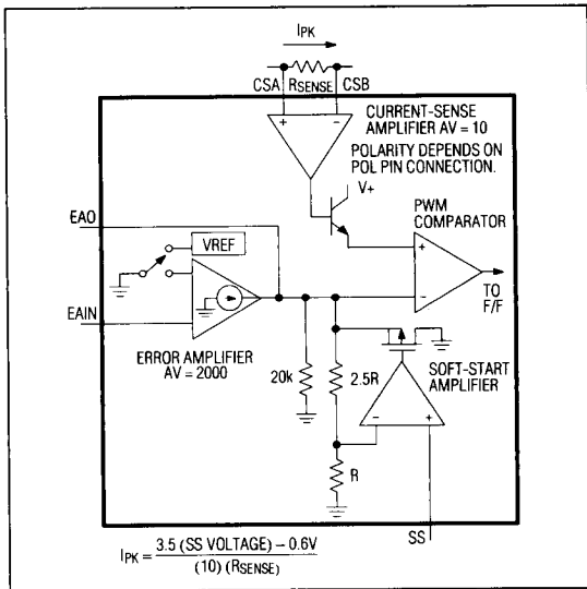
Figure 4. Soft-Start and Current Limit
