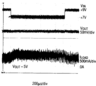
MAX741D STEP-DOWN LINE-TRANSIENT RESPONSE
