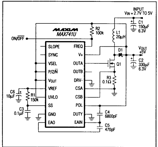
Figure 6. MAX741U EV Kit Schematic. This step-up converter supplies +5V at 1A from a +3V input.
