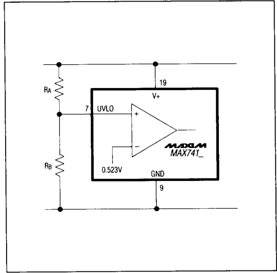
Figure 5. Undervoltage Lockout Comparator (Adjustable Mode)
