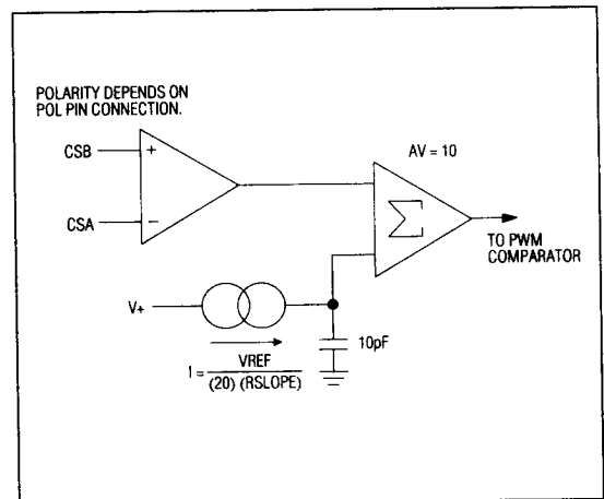
Figure 3. Current Amplifier and Slope Compensation Model
