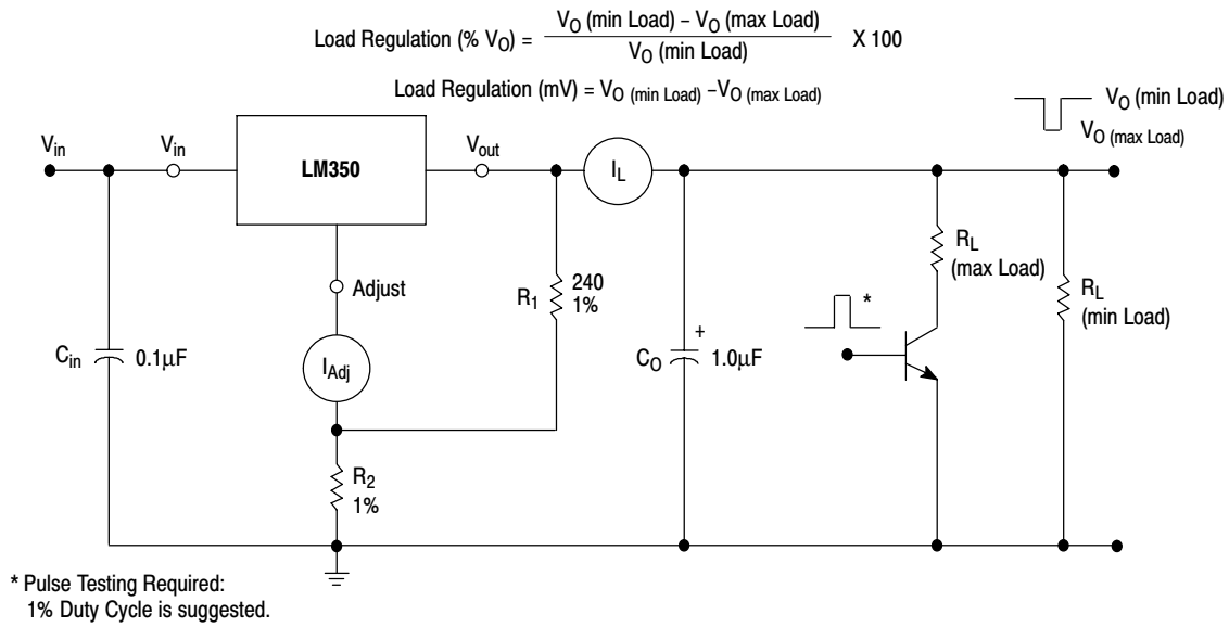
Figure 2. Load Regulation and \Delta I_{Adj}/\text{Load} Test Circuit
