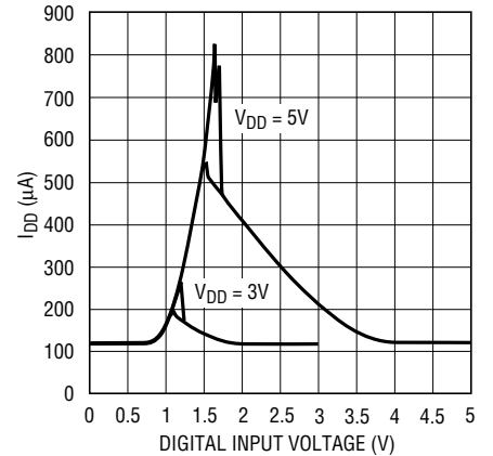
Supply Current ( I_{DD} ) vs Digital Input Voltage
