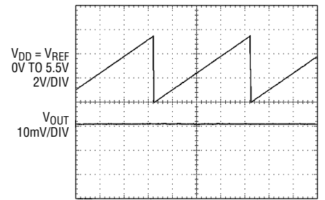
V_{OUT} vs V_{DD} = 0\text{V} to 5.5\text{V} (POR Function) LTC2641
