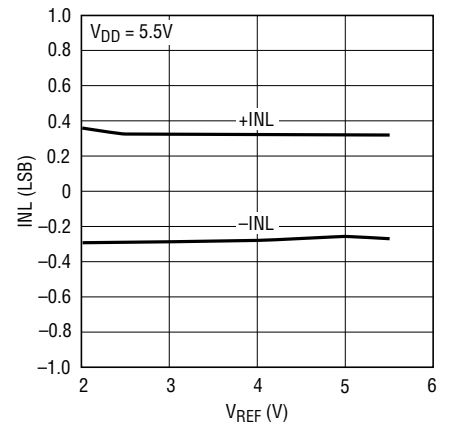
INL vs V_{REF}
