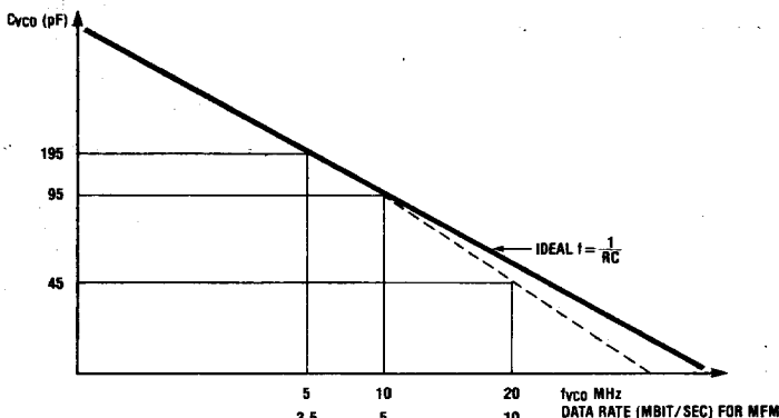
FIGURE 10. VCO Capacitor Value for Disk Data Rates
