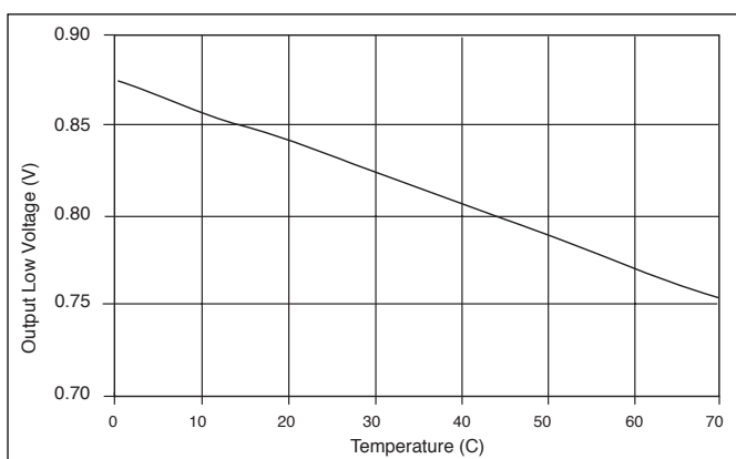
Figure 36: Error Amplifier Output Low Voltage ( 500\mu\text{A} ) vs Temperature.
