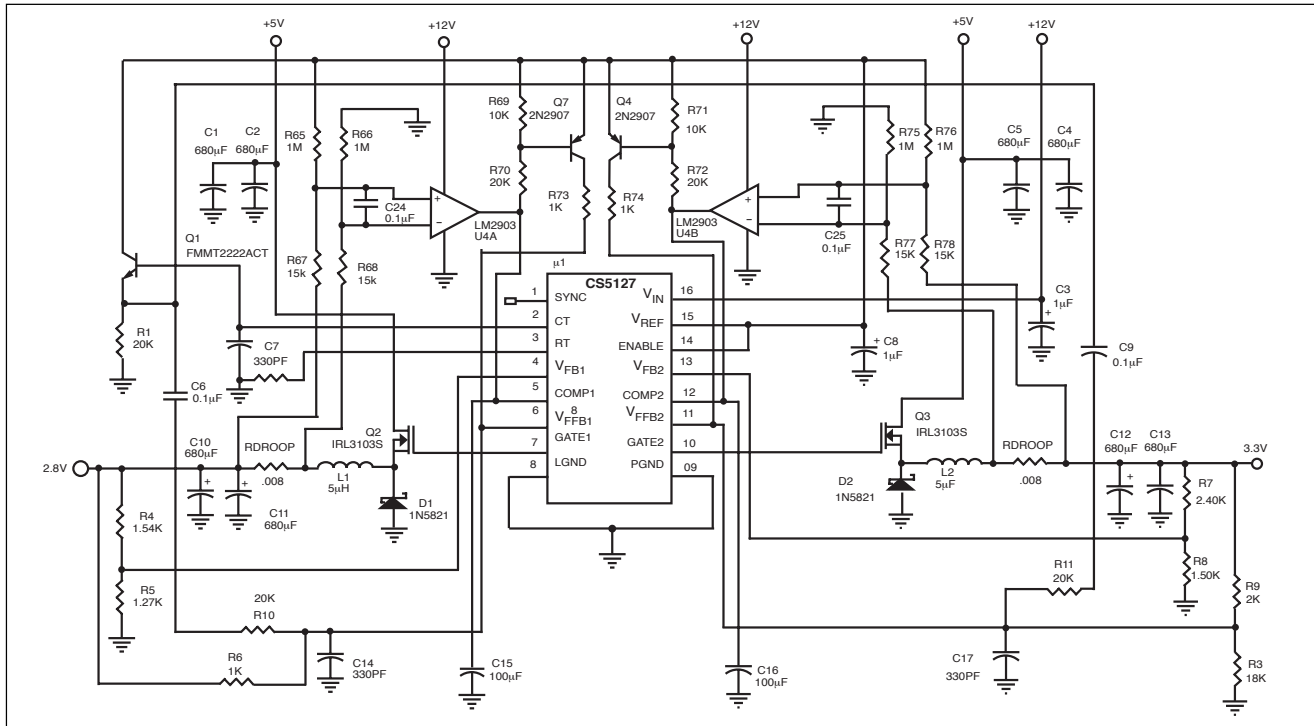
Figure 17: 200kHz, V 2 ™, 5V/12V input, 2.8V @ 7A and 3.3V @ 7A outputs with current limit.
