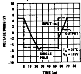
Voltage Follower Pulse Response
