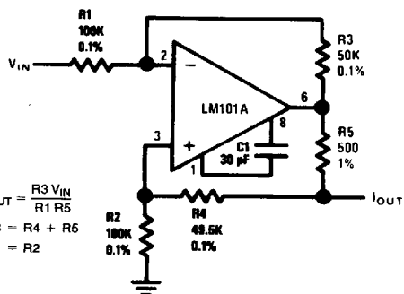
Bilateral Current Source
