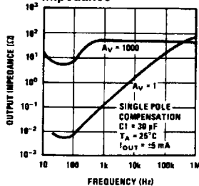
Closed Loop Output Impedance
