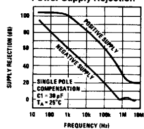
Power Supply Rejection
