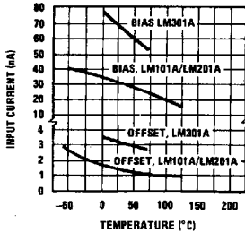
Input Current, LM101A/LM201A/LM301A
