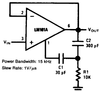
Fast Voltage Follower
