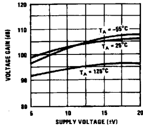
Voltage Gain
