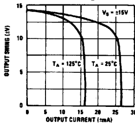
Current Limiting
