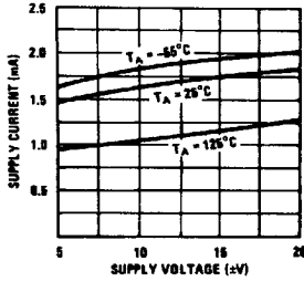
Supply Current
