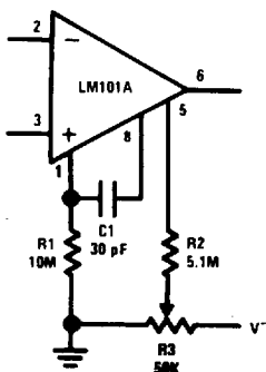
Standard Compensation and Offset Balancing Circuit
