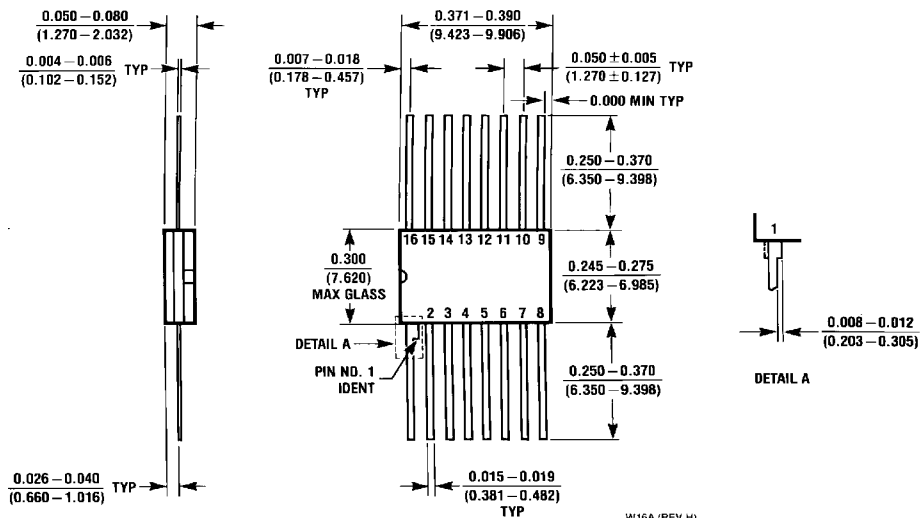
16-Lead Ceramic Flat Package (W) Order Number 54153FMBQ or DM54153W NS Package Number W16A
