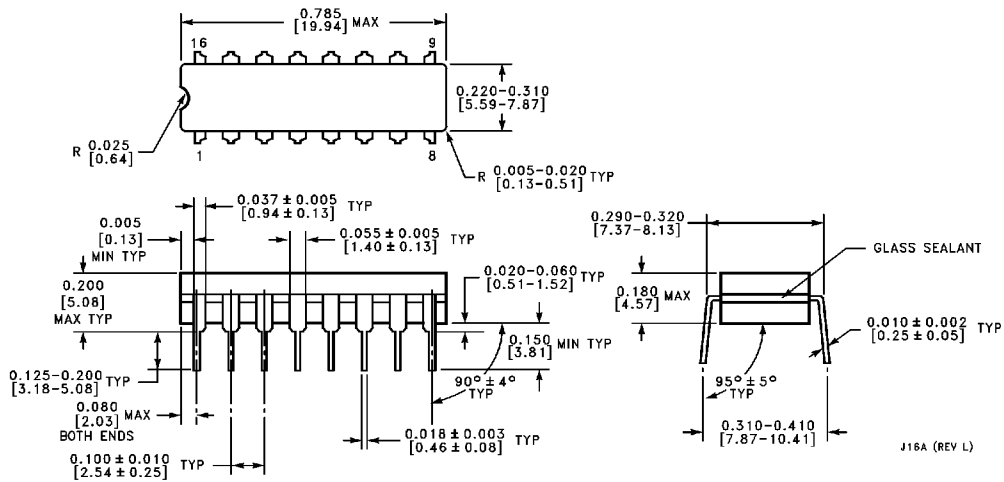
16-Lead Ceramic Dual-In-Line Package (J) Order Number 54153DMQB or DM54153J NS Package Number J16A
