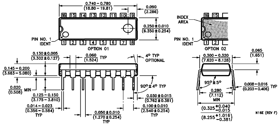
16-Lead Molded Dual-In-Line Package (N) Order Number DM74153N NS Package Number N16E
