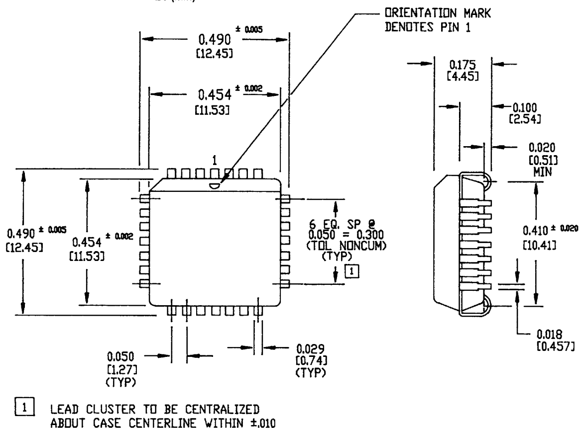
FIGURE 8. DD-03182PP: PLCC MECHANICAL OUTLINE
