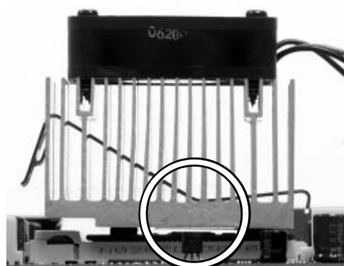
Photo 5. Proper location on processor
