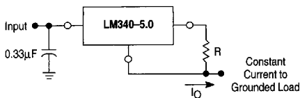
Figure 14. Current Regulator
