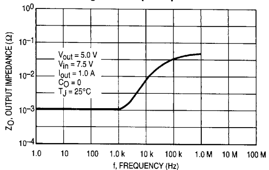
Figure 4. Output Impedance
