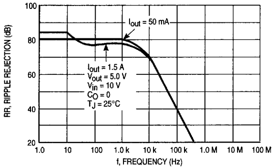
Figure 5. Ripple Rejection versus Frequency
