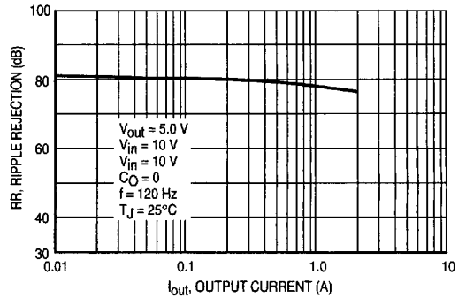
Figure 6. Ripple Rejection versus Output Current
