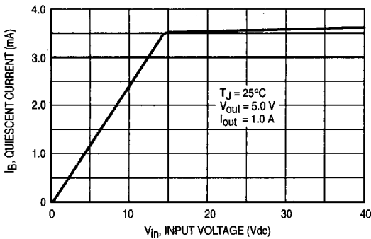
Figure 7. Quiescent Current versus Input Voltage
