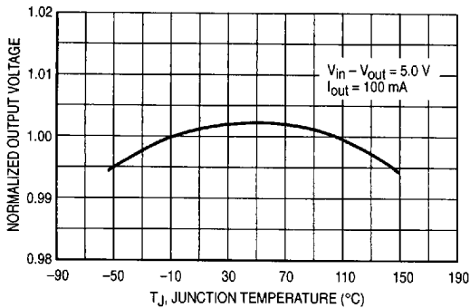
Figure 3. Temperature Stability
