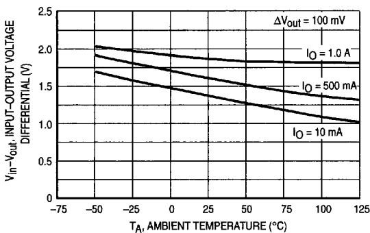
Figure 9. Dropout Voltage
