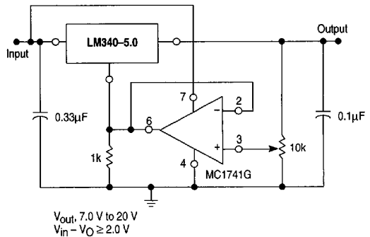
Figure 15. Adjustable Output Regulator
