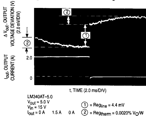
Figure 2. Load and Thermal Regulation
