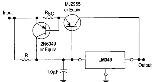
Figure 17. Short Circuit Protection
