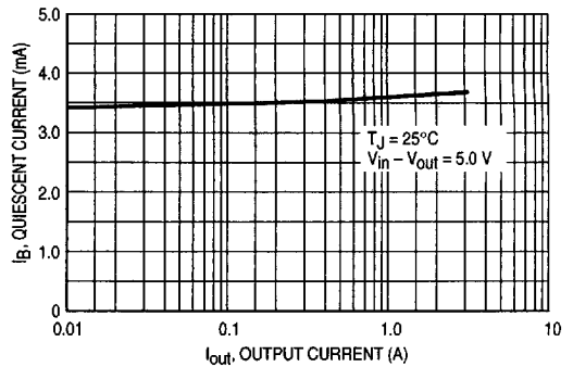
Figure 8. Quiescent Current versus Output Current
