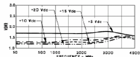
Input VSWR vs. Frequency
