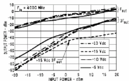
Limiting Characteristics
