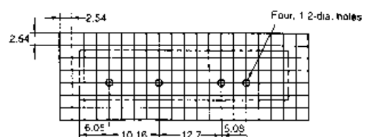
Terminal Arrangement (Bottom View)
