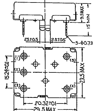
Mechanical Dimensions of LG / LGH Series
