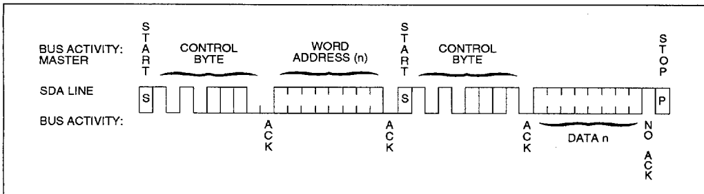
FIGURE 9-2: RANDOM READ
