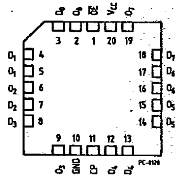
CHIP CARRIER
