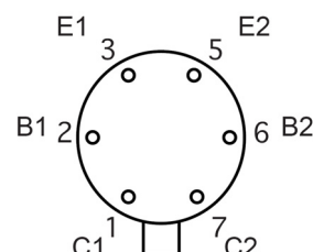
TO-71 (Bottom View)
