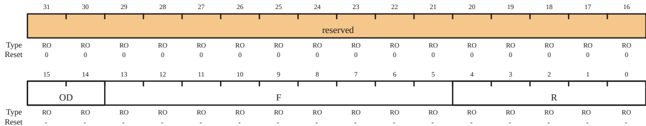
XTAL to PLL Translation (PLLCFG) Offset 0x064
