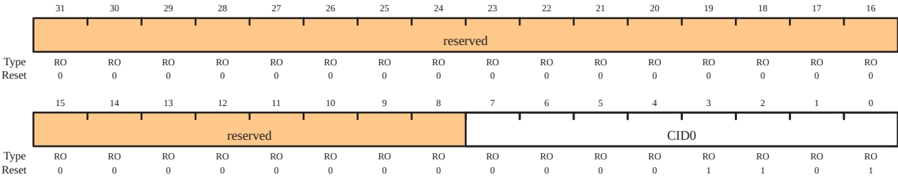
GPIO Primecell Identification 0 (GPIOCellID0) Offset 0xFF0
