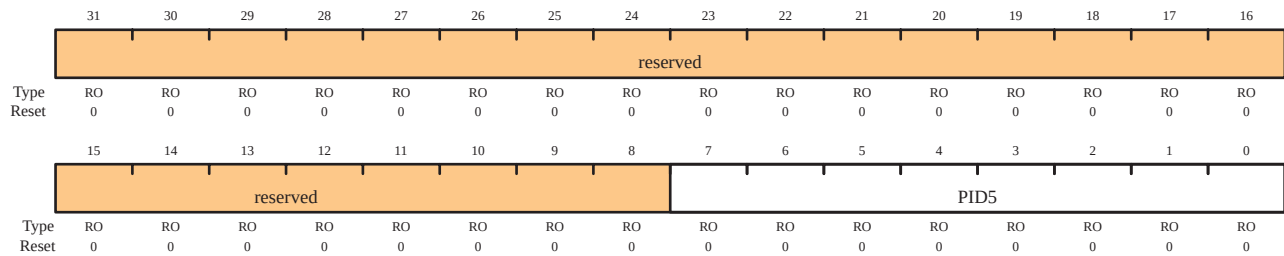
GPIO Peripheral Identification 5 (GPIOPeriphID5)
