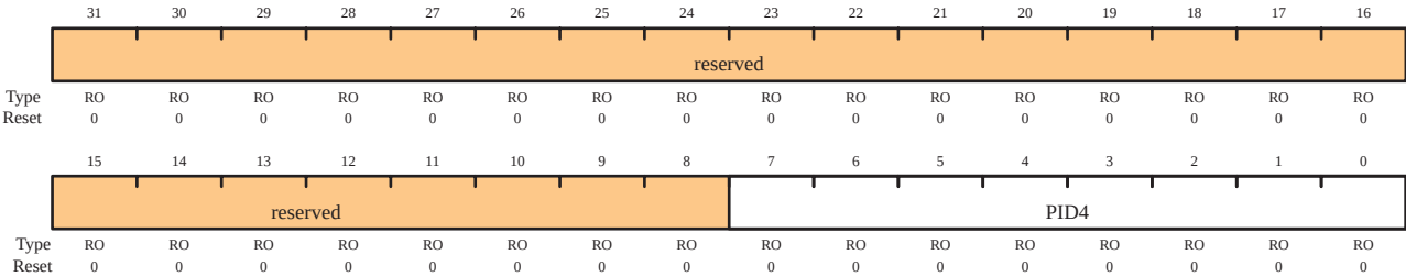
GPIO Peripheral Identification 4 (GPIOPeriphID4)
