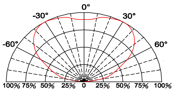
Fig.5 Directive Radiation
