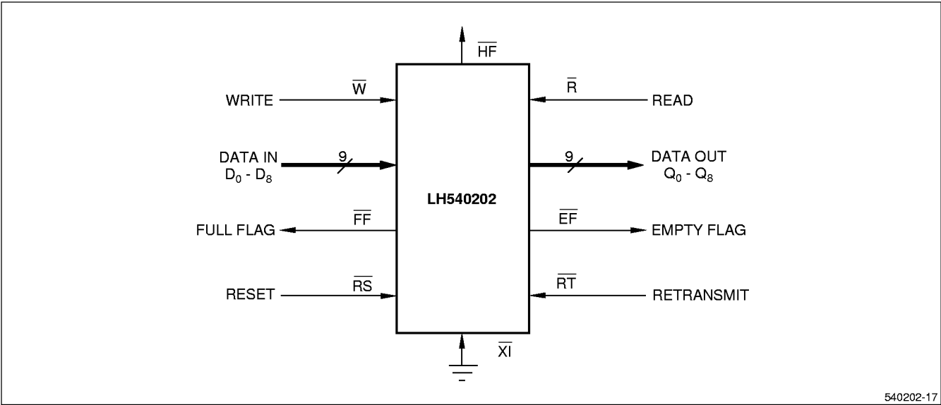
Figure 4. Standalone FIFO (1024 × 9)
