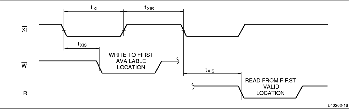
Figure 21. Expansion-In Timing
