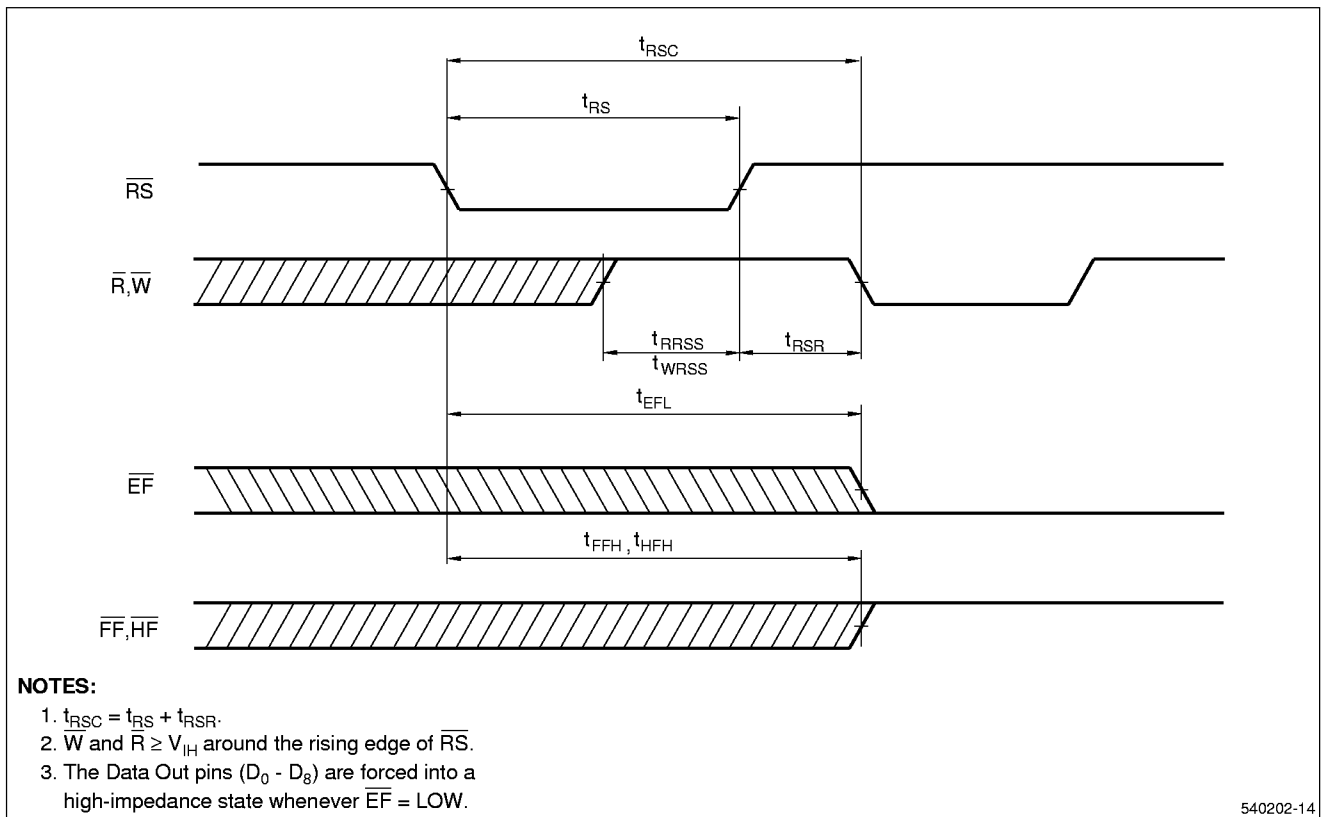
Figure 10. Reset Timing
