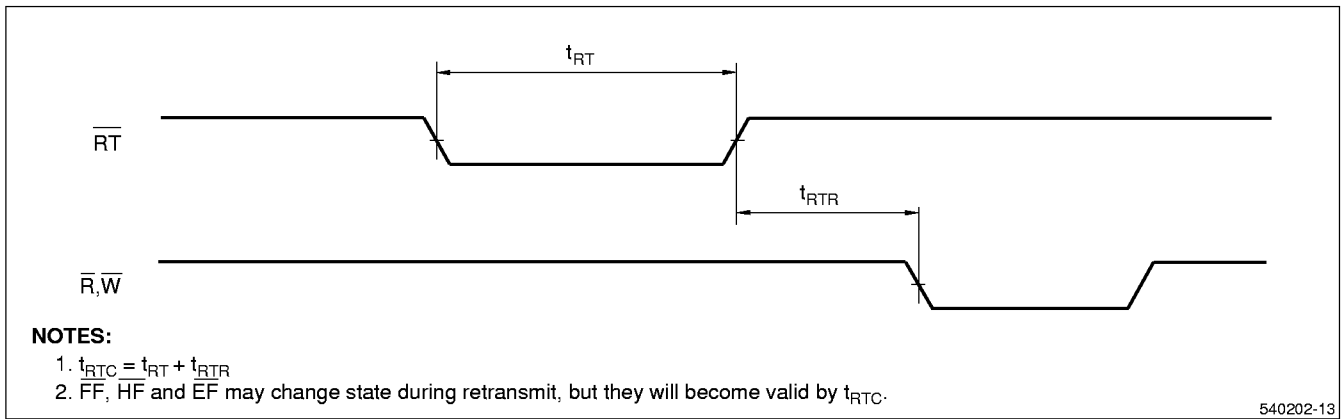
Figure 19. Retransmit Timing
