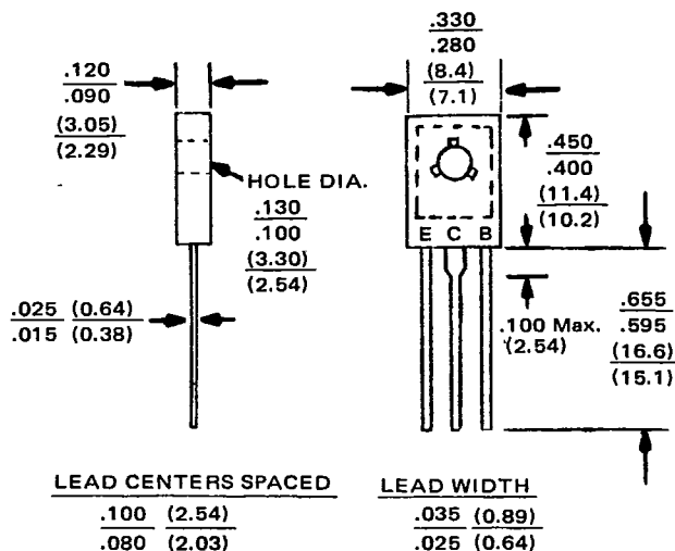
To-126
