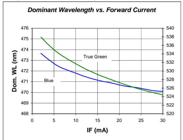
Fig. 6 Dominant Wavelength vs. Forward Current
