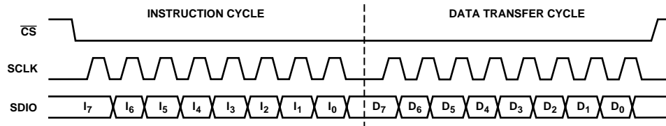
Figure 34. Serial Port Writing Timing—Clock Stall Low
