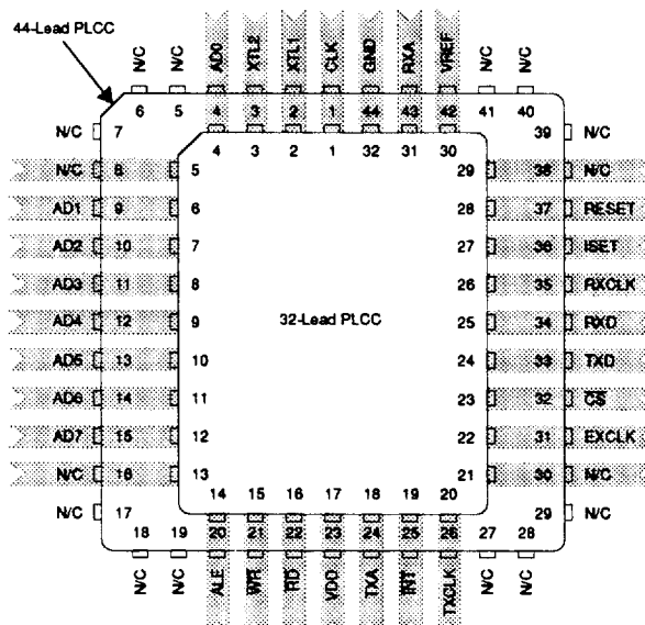
32, 44-Lead PLCC
