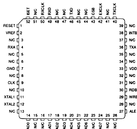
52-Lead QFP
