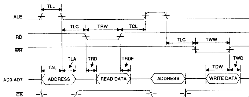
BUS TIMING DIAGRAM (PARALLEL VERSION)
