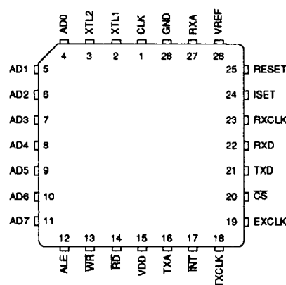
28-Lead PLCC
