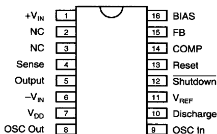
16 Pin Dip Package top view
