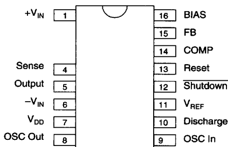
16 Pin SOIC top view
