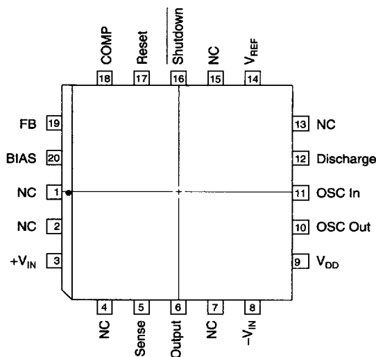
20-pin PJP Package top view
