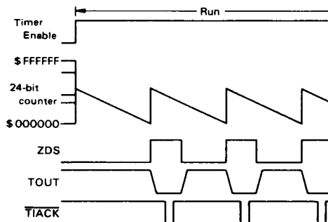
Figure 20 Periodic Interrupt Generator
