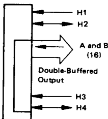
Figure 15 Mode 1 Port B Submode X1
