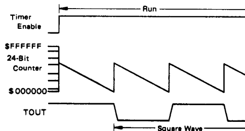
Figure 21 Square Wave Generator
