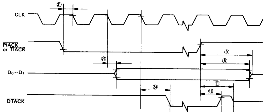
Figure 4 Interrupt Acknowledge Functional Timing Diagram
