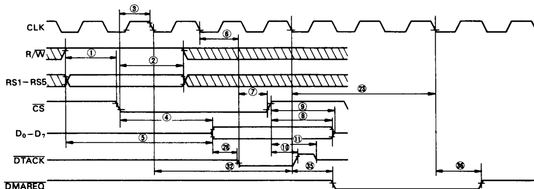
Figure 2 Bus Read Cycle Timing
