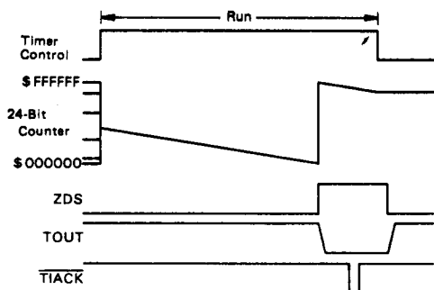
Figure 22 Interrupt After Timeout
