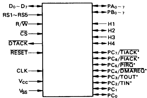
Figure 7 Input and Output Signals
