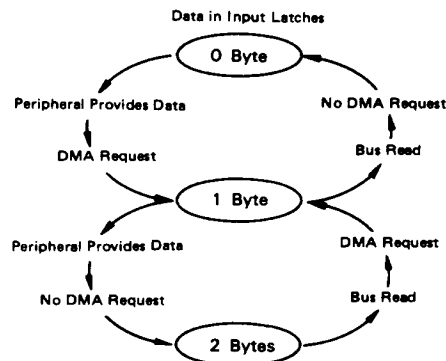
Figure 19 DMAREQ Associated with Input Transfers
