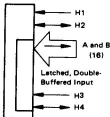
Figure 14 Mode 1 Port B Submode X0
