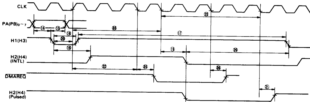
Figure 5 Peripheral Interface Input Timing
