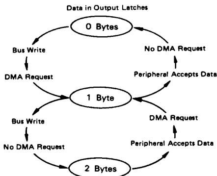
Figure 18 DMAREQ Associated with Output Transfers
