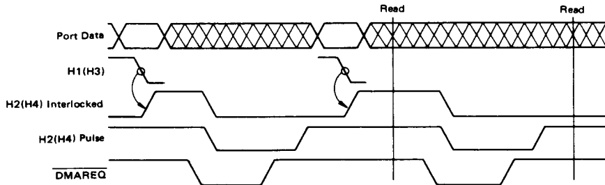
Figure 9 Double-buffered Input Transfers
