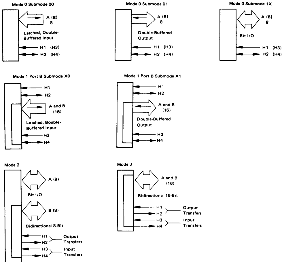
Figure 8 Port Mode Layout
