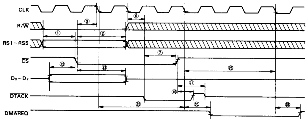
Figure 3 Bus Write Cycle Timing
