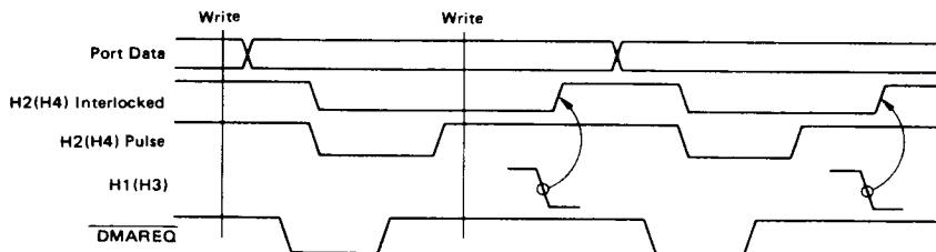
Figure 10 Double-buffered Output Transfers
