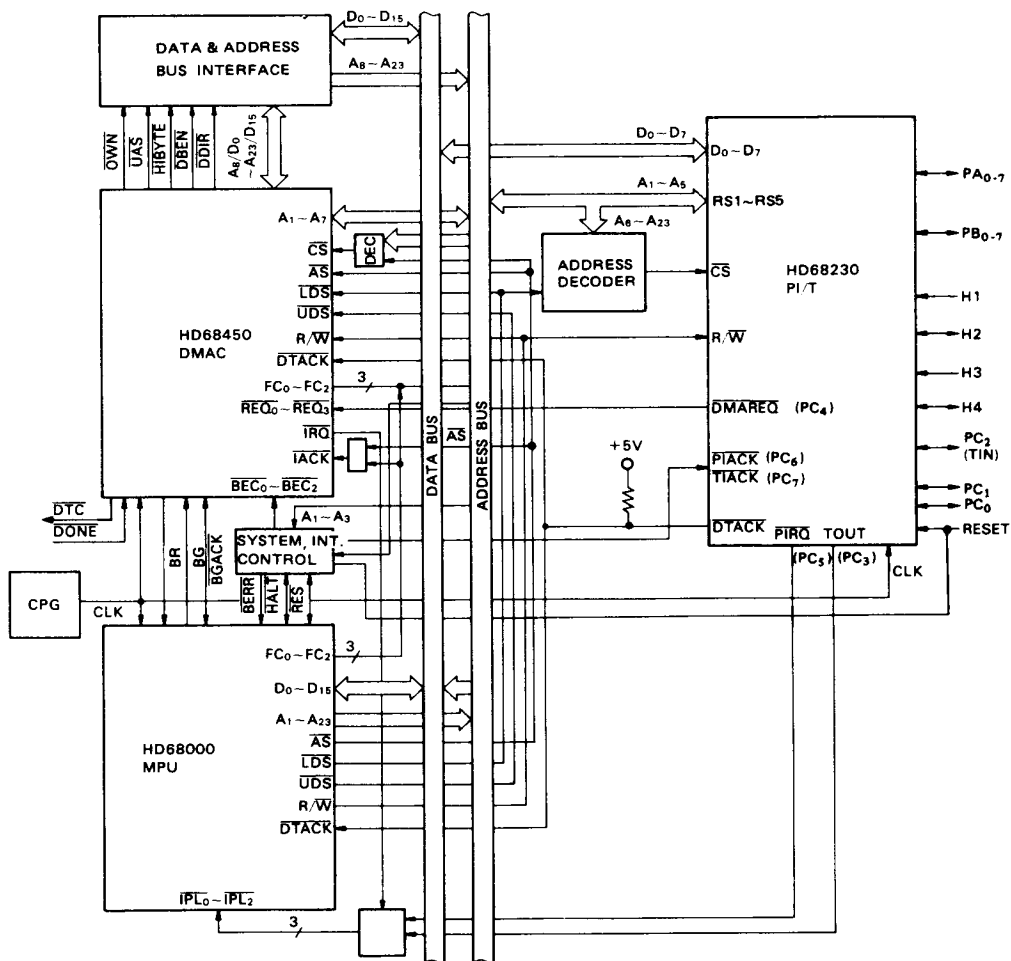
Figure 25 HD68000 Interface-Example
