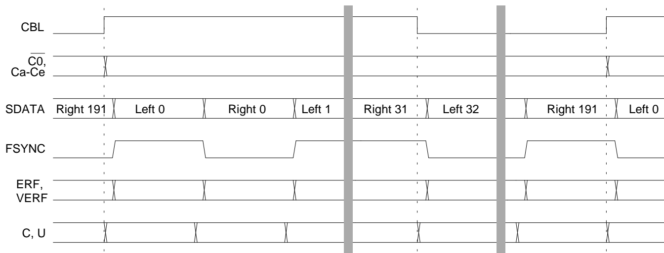
Figure 19. CBL Timing
