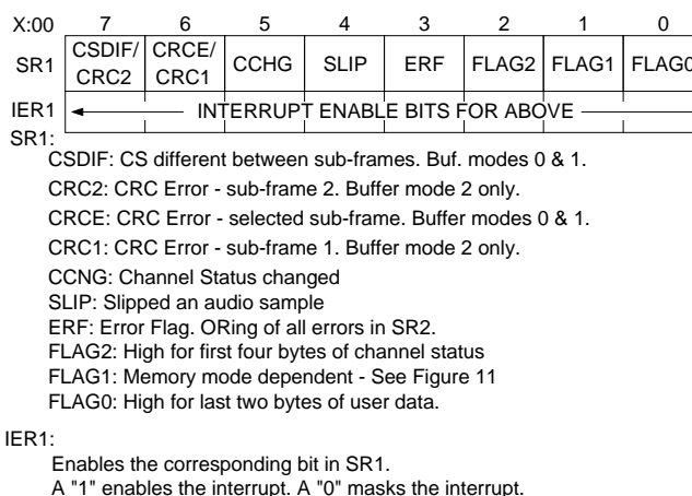
Figure 6. Status/IEnable Register 1
