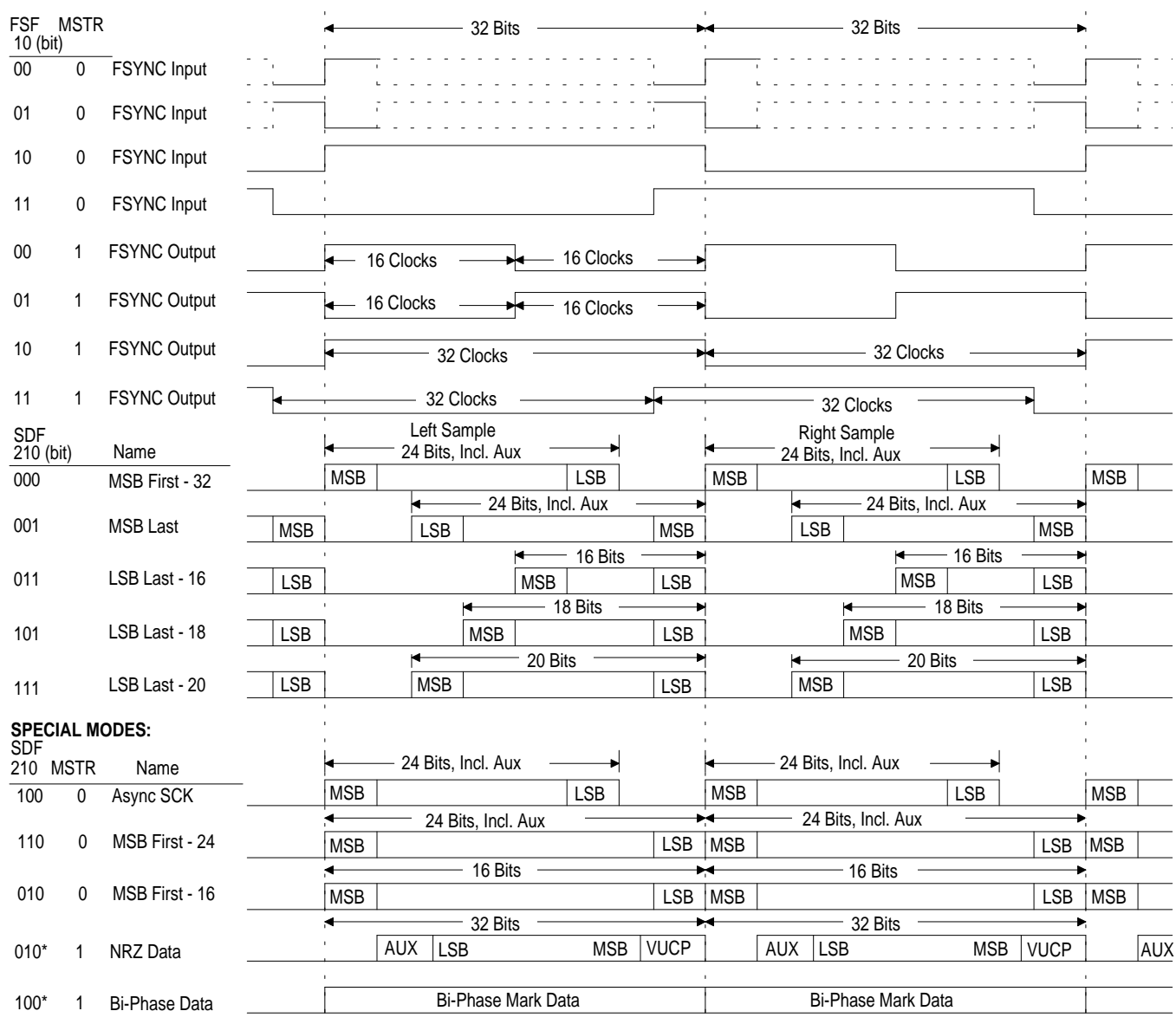
Figure 10. CS8411 Serial Port SDATA and FSYNC Timing
