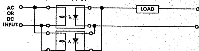
FIGURE 3. Full-wave AC switching (normally open) (AC load supply).
