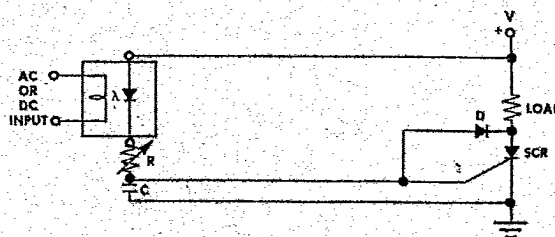
FIGURE 16. Isolated time delay relay (DC load supply).
