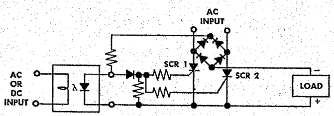
FIGURE 7. High power DC switching (normally closed) (AC load supply).
