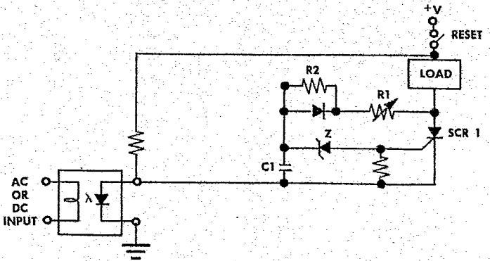
FIGURE 8. Time delayed high power DC switching (normally open) (DC load supply).
