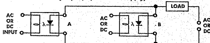
FIGURE 10. "OR" logic control (normally open) (AC or DC load supply).
