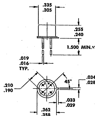
OUTLINE DIMENSIONS
