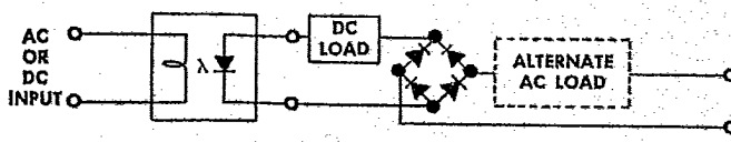
FIGURE 5. Full-wave AC or DC switching (normally open) (AC load supply).
