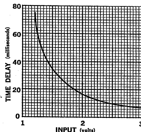
TIME DELAY CHARACTERISTIC
