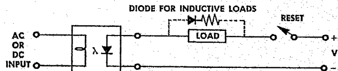
FIGURE 1. DC switching (normally open) (DC load supply).
