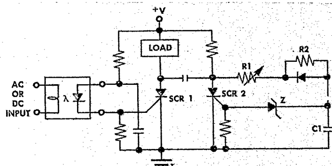
FIGURE 9. Time interval high power DC switching (normally open) (DC load supply).
