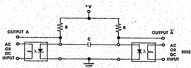
FIGURE 13. Control Flip-Flop (DC load supply).
