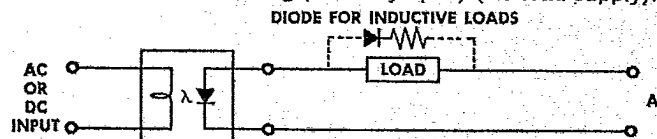
FIGURE 2. Half-wave AC switching (normally open) (AC load supply).
