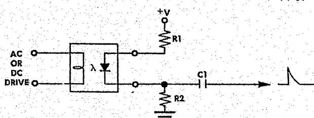
FIGURE 15. Positive pulse generator (DC load supply).
