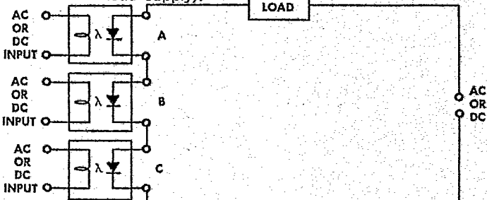
FIGURE 11. "AND" logic control (normally open) (AC or DC load supply).
