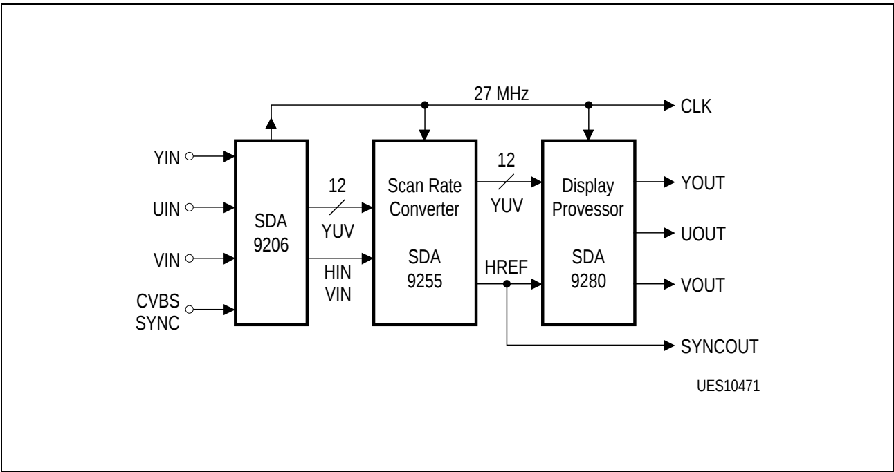
Figure 19 Application Circuit 2
