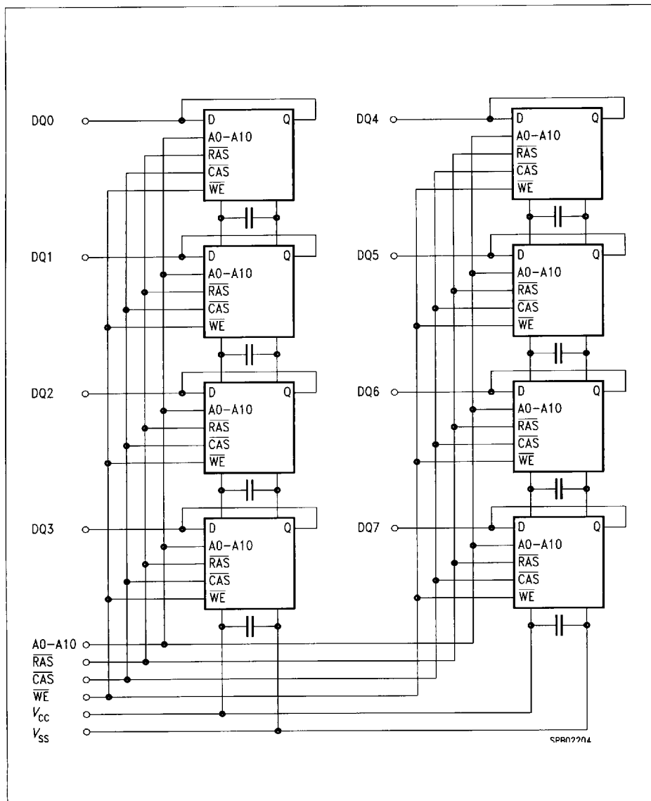
Block Diagram
