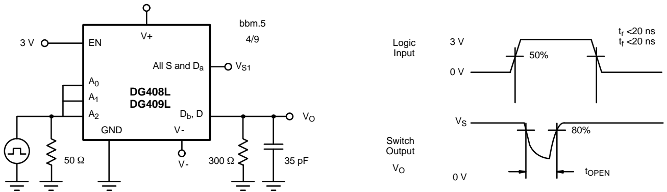
FIGURE 4. Break-Before-Make Interval
