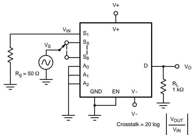
FIGURE 7. Crosstalk
