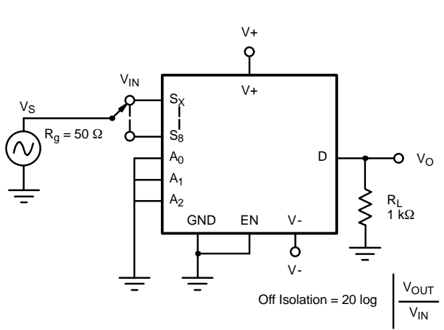
FIGURE 6. Off Isolation
