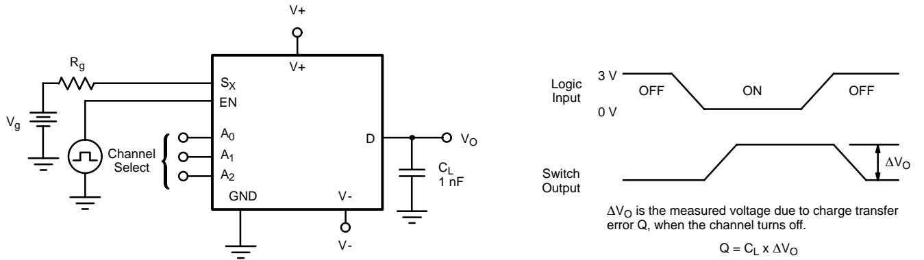
FIGURE 5. Charge Injection
