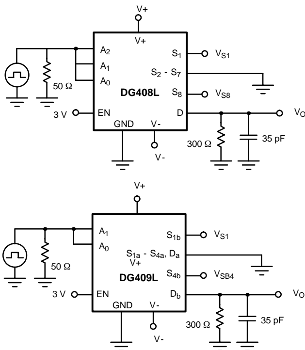
FIGURE 2. Transition Time
