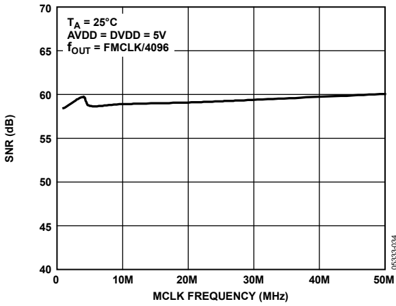
Figure 15. SNR vs. MCLK Frequency
