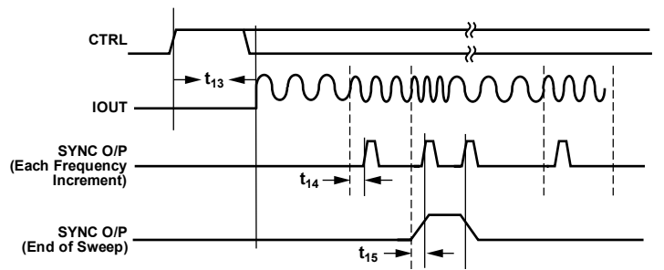
Figure 6. CTRL Timing, Saw-Sweep Mode
