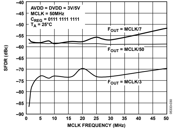
Figure 12. Wideband SFDR vs. MCLK Frequency
