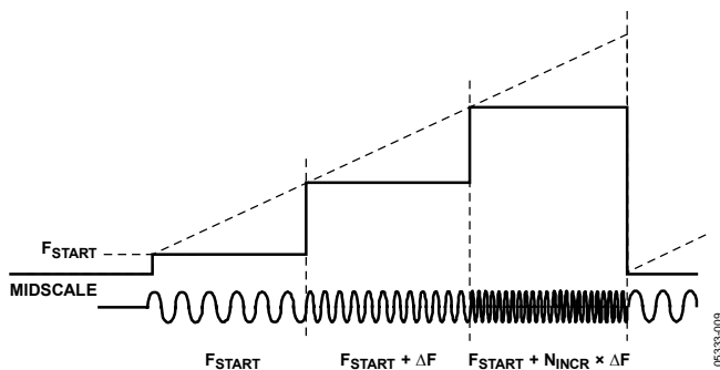
Figure 31. Saw-Sweep Profile
