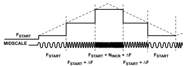
Figure 32. Triangular-Sweep Profile
