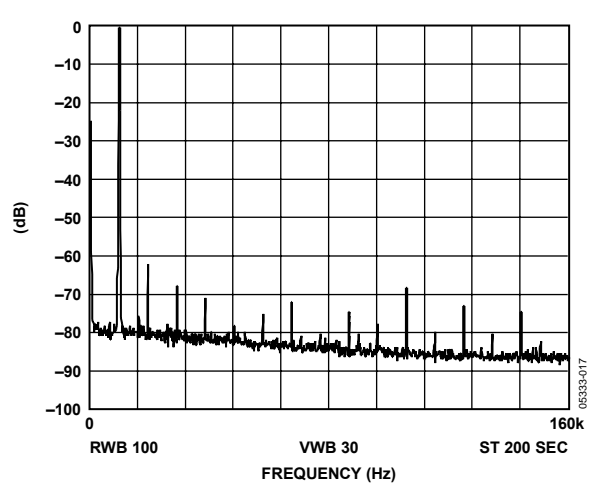
Figure 25. f_{MCLK} = 50 \text{ MHz} ; f_{OUT} = 12 \text{ kHz} , Frequency Word = 000FBA9
