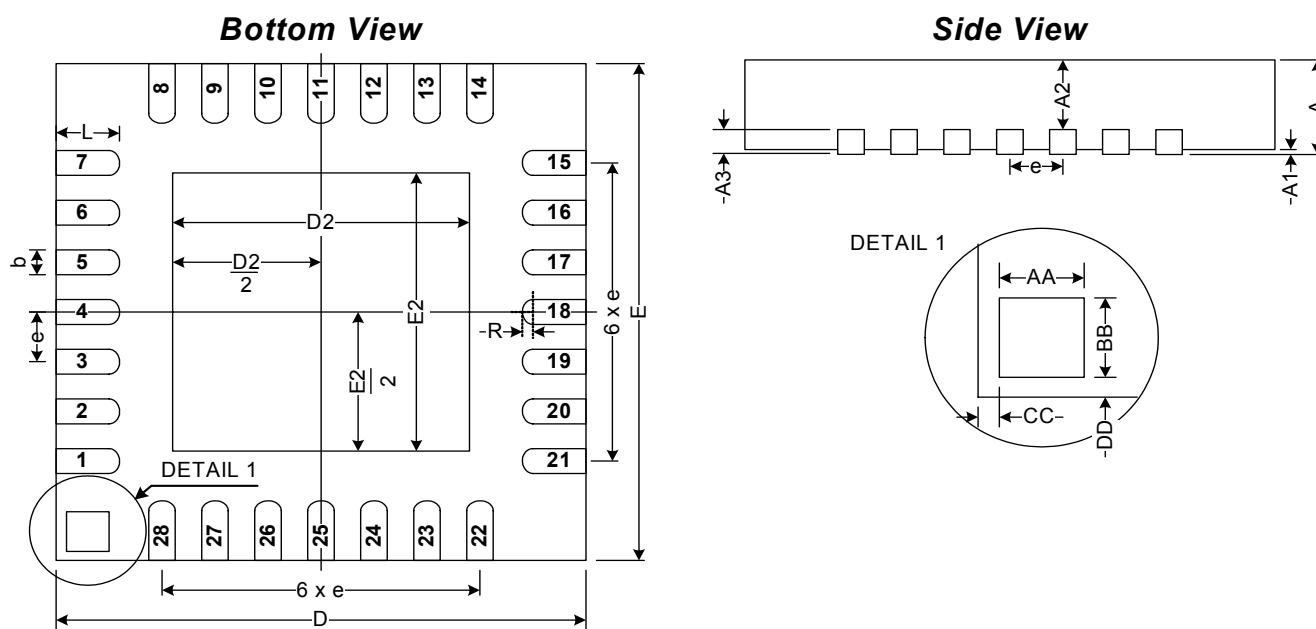
Figure 14. 28-lead Quad Flat No-lead (QFN) Package Diagram
