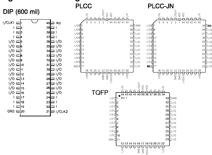
Figure 1: Pin Configuration
