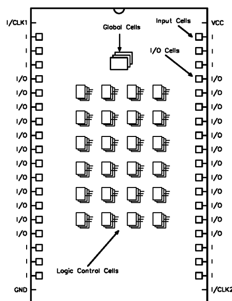
Figure 2: Block Diagram
