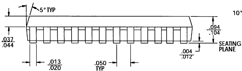
24-Pin SOIC (S24)
