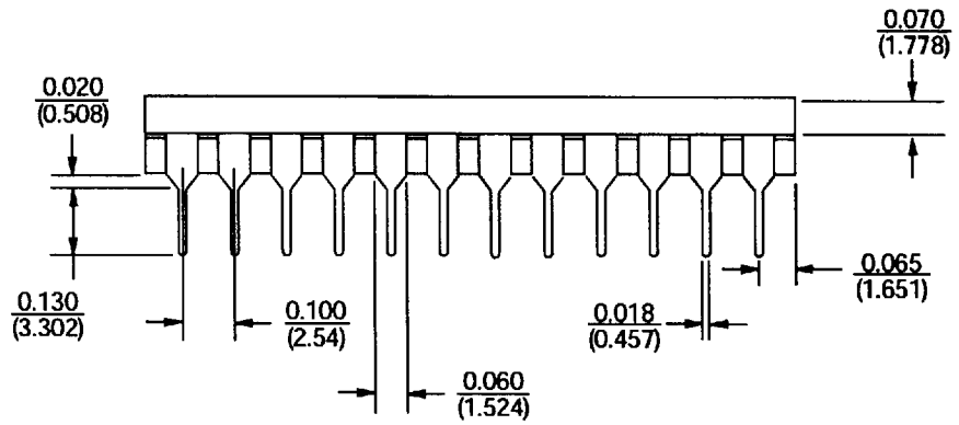
24-Pin Plastic DIP (P24)
