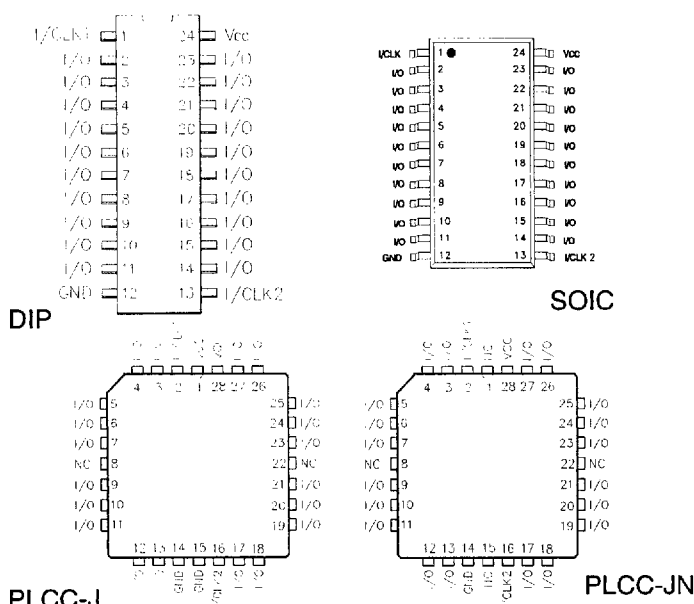
Figure 1: Pin Configuration
