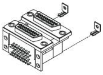
SINGLE BOARDLOCK
