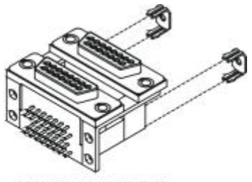
DUAL BOARDLOCKS
