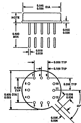
To-8 BOTTOM VIEW
