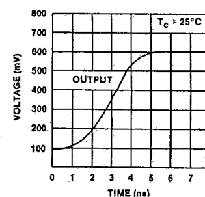
SMALL SIGNAL RISE TIME
