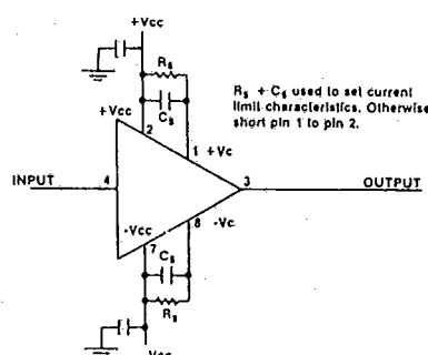
TYPICAL CIRCUIT 330
