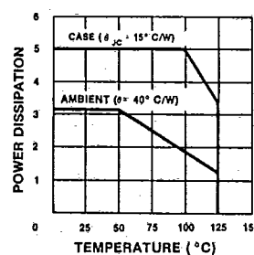
To-3 POWER DISSIPATION
