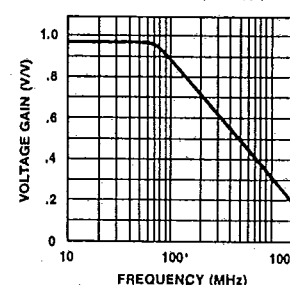
FREQUENCY RESPONSE
