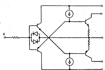
SCHEMATIC 330
