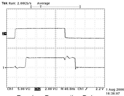
Receiver Propagation Delay (SP3086-SP3088)
